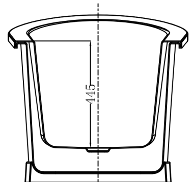
SECTION E-E
